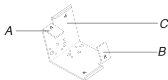
A. P Hook B. R Hook C. P and R Bracket
